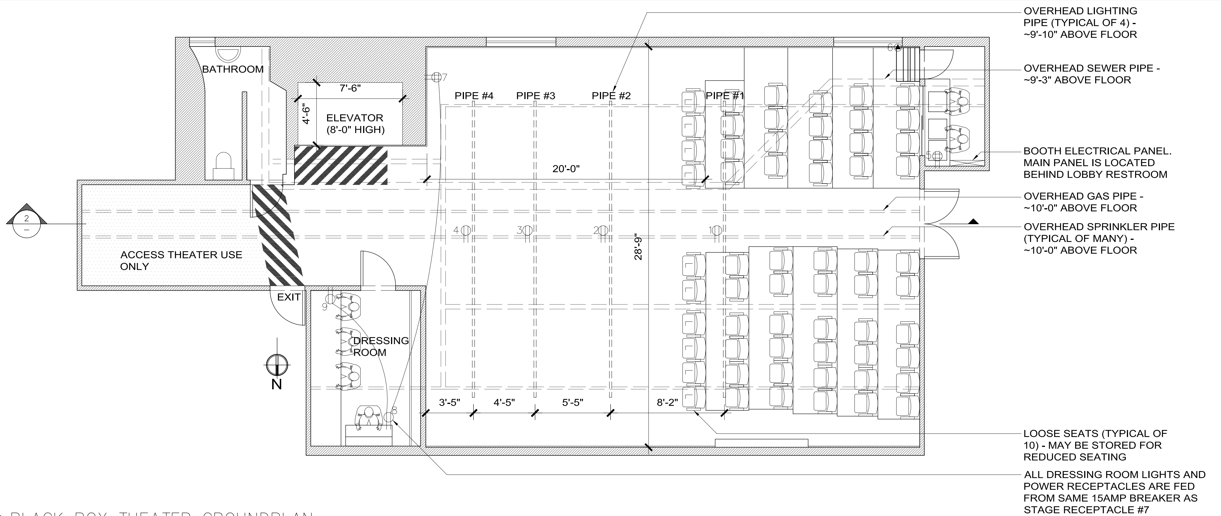
1 BLACK BOX THEATER GROUNDPLAN 1/4" = 1'-0"
